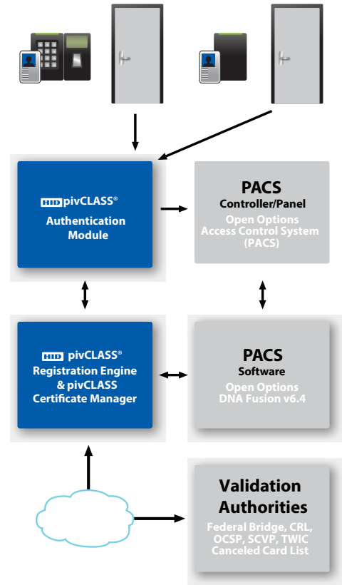
pivCLASS® System Diagram
